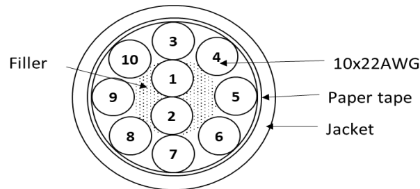
Fig. 1 Cross-section of cable
